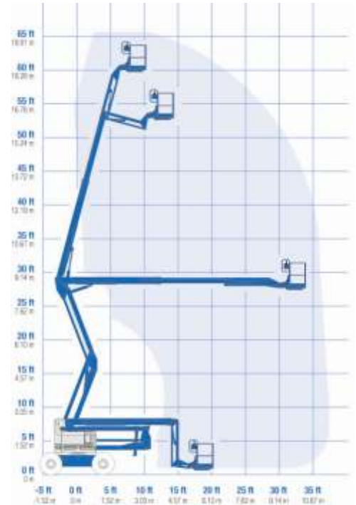
Genie Z60/34 2427, 2577, 2581
